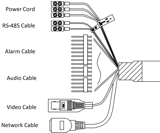
Figure 1-3 Cable Interfaces
